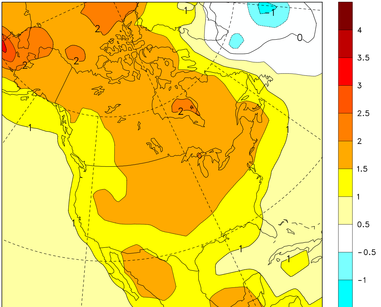
Surface Air Temp, C, change, SRESB1/T47 ANN 2041-2060 vs 1981-2000
